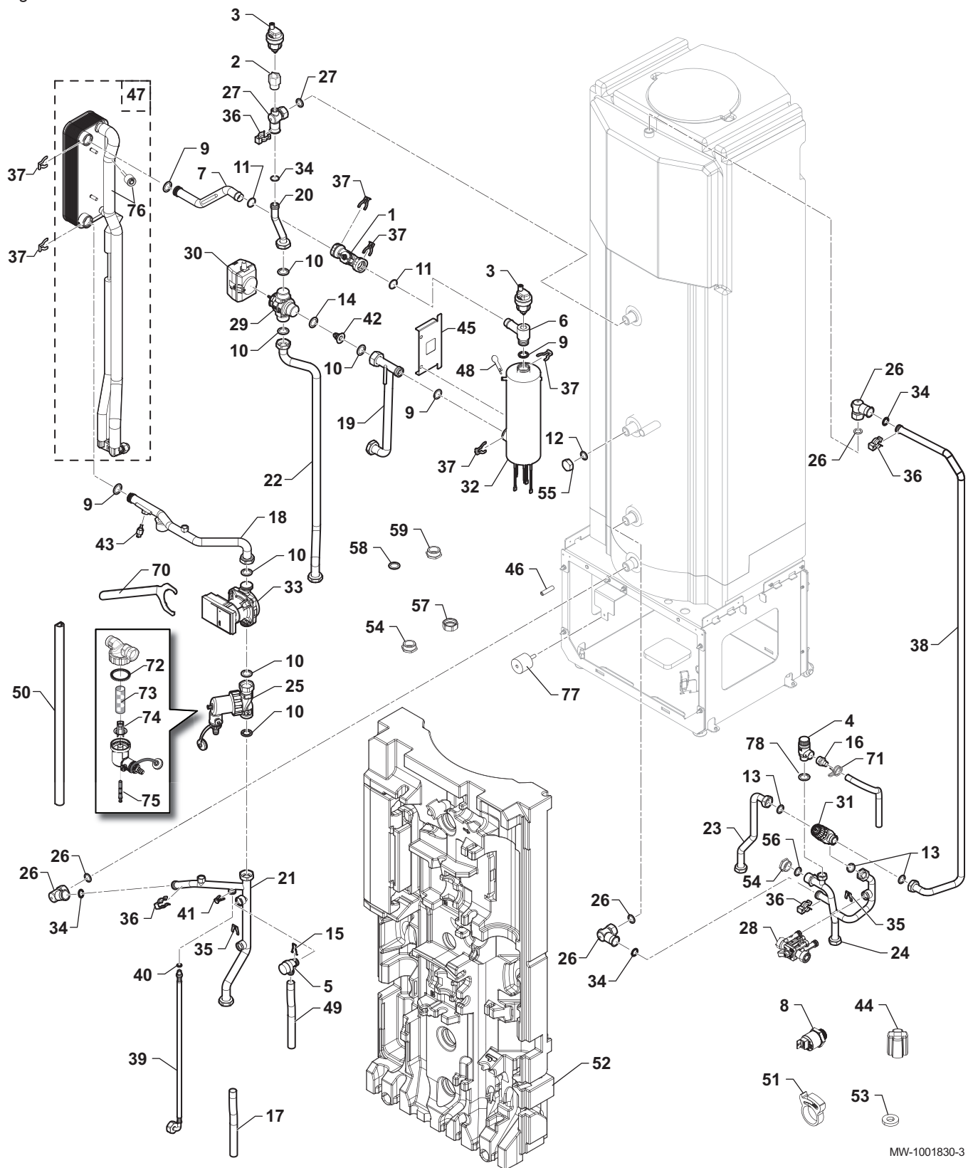
Fig.158 Circuit A
